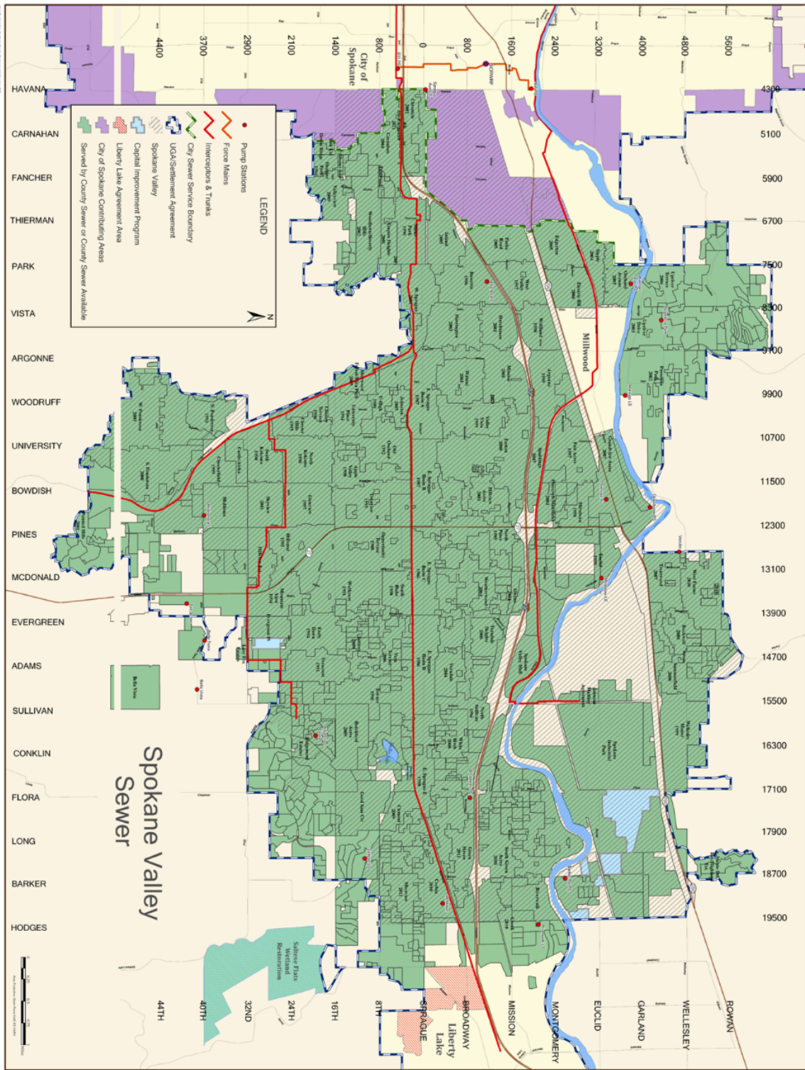
Map CF-04: Spokane Valley Sewer Basins
