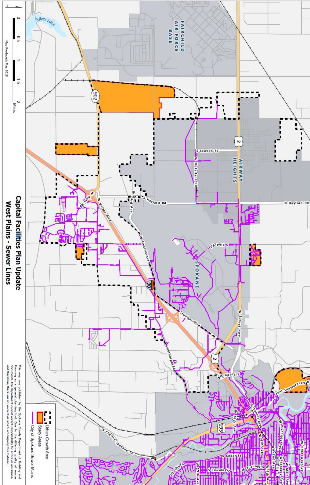
Map CF-07: West Plains Sewer Mains
