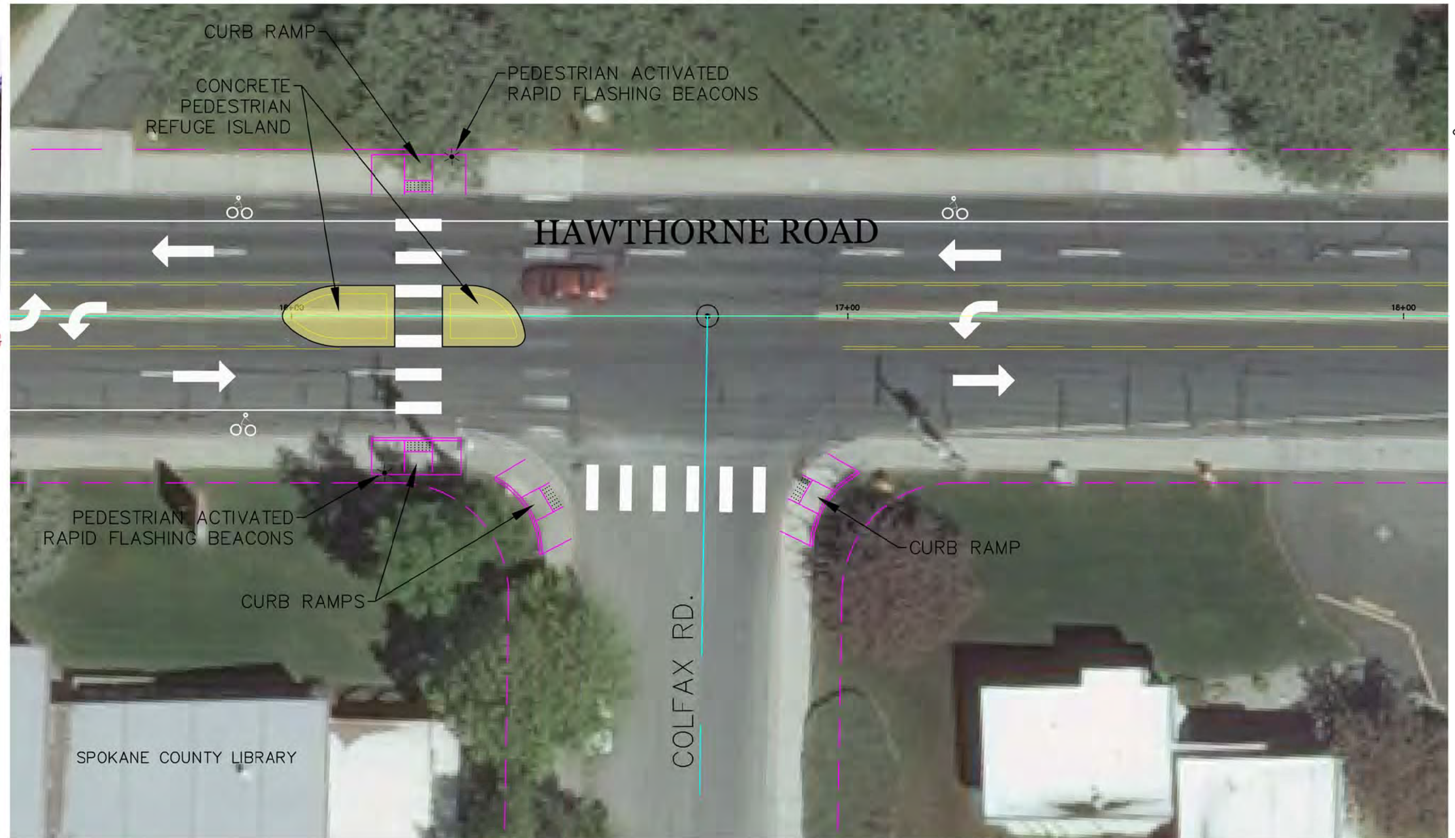
PEDESTRIAN ACTIVATED RAPID FLASHING BEACON
