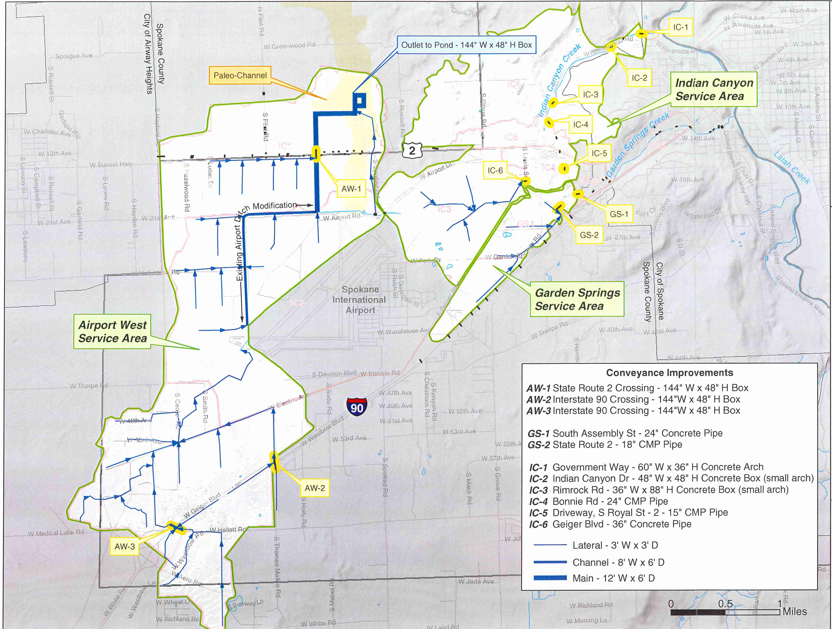
Figure 3-6 Service Areas and Potential Conveyance Improvements
