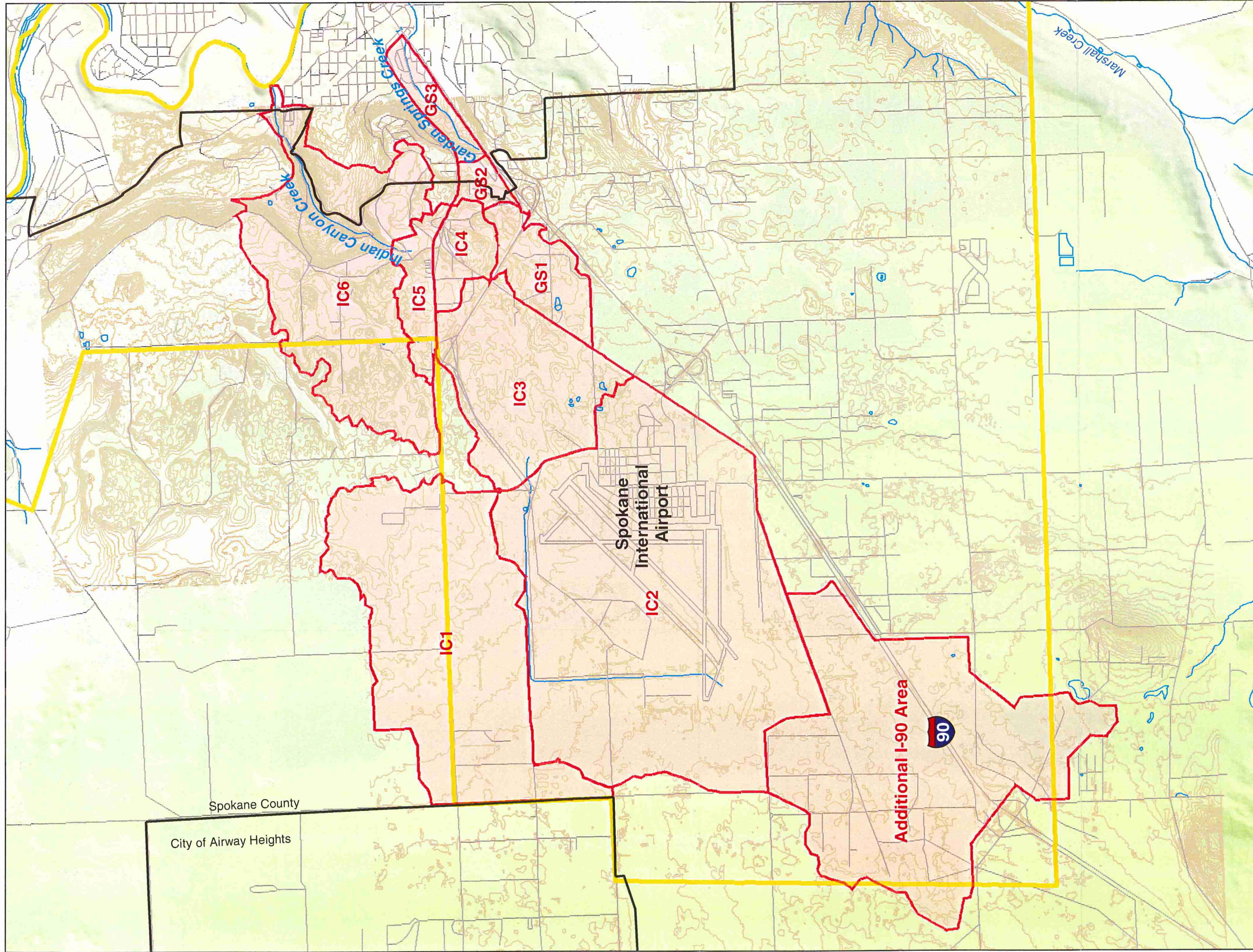
Figure 3-5 Sub-Basins Used in HSPF Analysis
