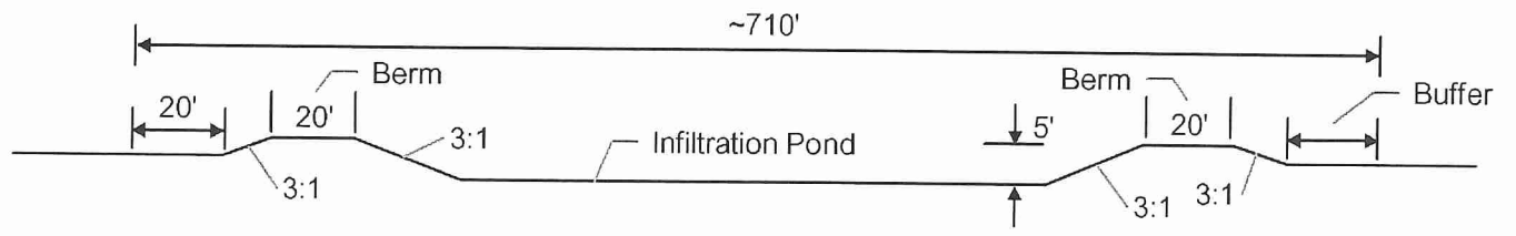
Figure 3-8 Conceptual Regional Infiltration Facility at Northern Paleo-Channel
