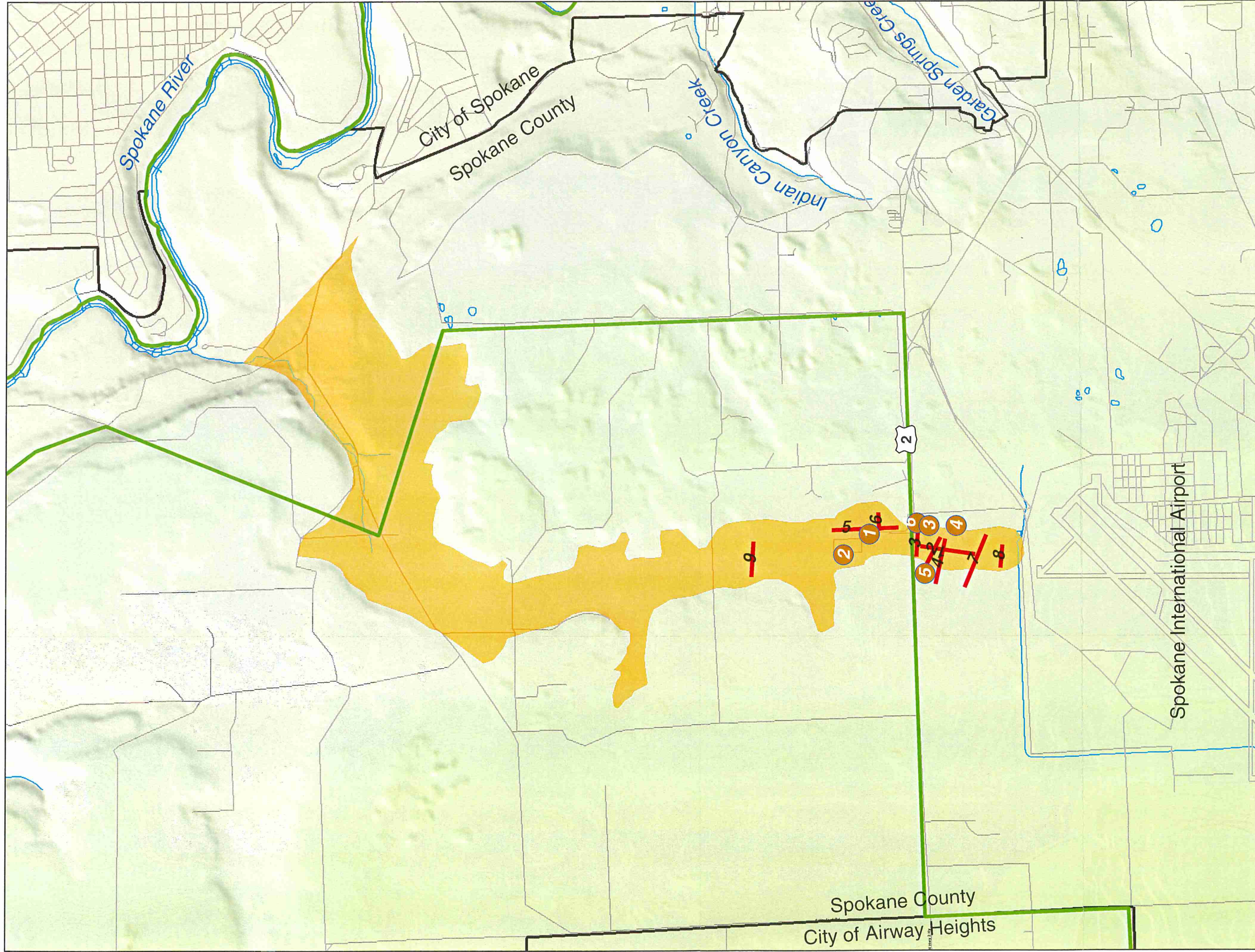
Figure 3-3 Paleo-Channel North of Airport with Seismic Survey Lines
