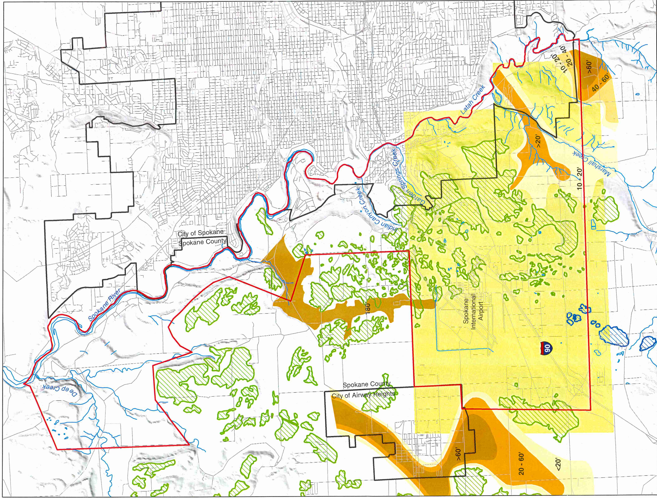
Figure 2-1 Planning Area Overburden Depth and Paleo-Channel Location
