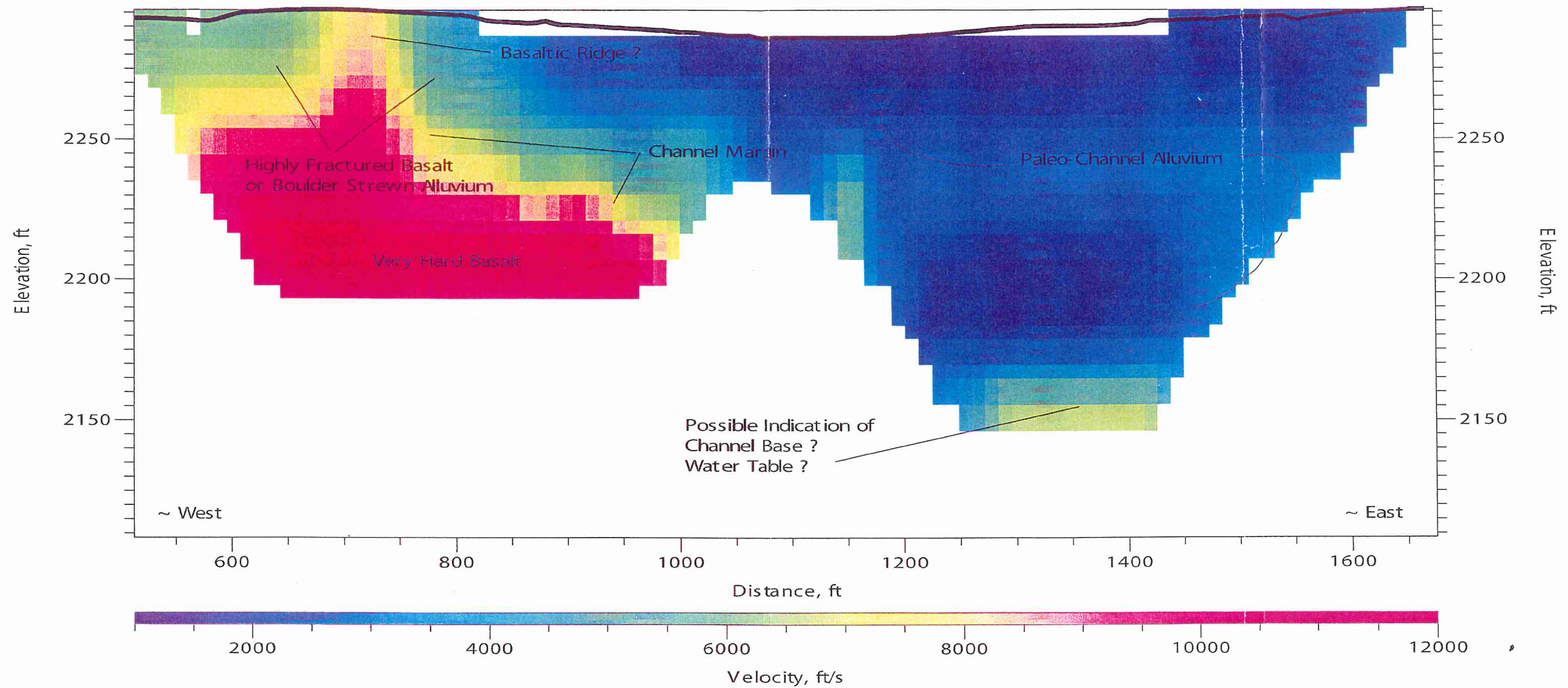
Velocity Model: Line 4
