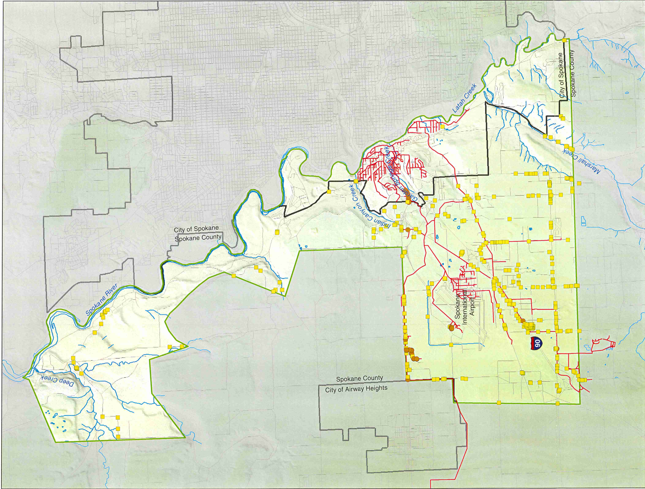
Figure 2-3 Known West Plains Stormwater Management Facilities
