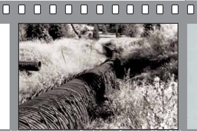
Wood stave pipe, Rathdrum Prairie, ID 1961
